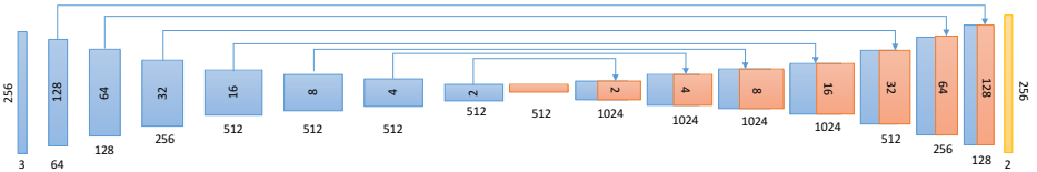
Fig. 9: Embedding Network : In the encoder, each convolution is followed by a leaky ReLU with factor 0.2 and then a batch-norm layer (except for the first which has no batch-norm). The convolutional filter sizes are 4 \times 4 and the stride/padding is 2/1. In this decoder, the layers from the encoder are concatenated using skip connections, doubling the channel size. In the decoder, the sequence of executions following each convolutional layer is: ReLU, bilinear up-sampling, batch-norm, concatenation (with the corresponding encoder layer). The last layer (yellow) does not have a concatenation. The final 2 \times 256 \times 256 result is passed through a tanh layer to give X2Face’s prediction for how to sample from the source frames. The convolutional filter sizes in the decoder are 3 \times 3 and the stride/padding is 1/1.
