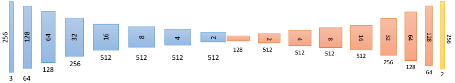
Fig. 10: Driving Network : The encoder is similar to the encoder of the embedding network ; each convolution is followed by a leaky ReLU (factor 0.2) and then a batch-norm layer (except for the first which has no batch-norm); the convolutional filter sizes are 4 \times 4 and the stride/padding is 2/1. In this decoder, there are no skip connections. The driving vector has channel size 128. In the decoder, the sequence of executions following each convolutional layer is: ReLU, bilinear upsampling, batch-norm. The final 2 \times 256 \times 256 result is passed through a tanh layer to give X2Face’s prediction for how to sample from the embedded face. The convolutional filter sizes in the decoder are 3 \times 3 and the stride/padding is 1/1.
