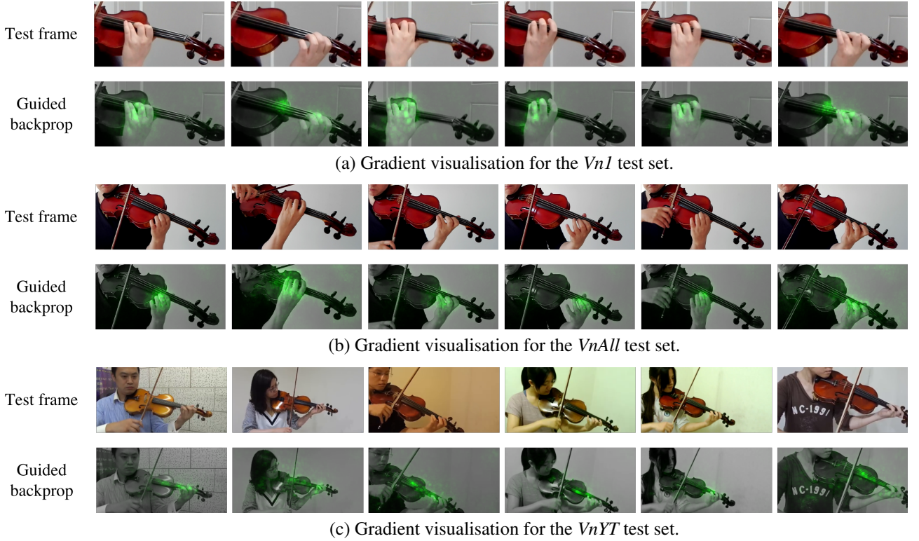
Figure 4. Discriminative information visualisations using guided backpropagation [23] for the test sets of the VnI subset in (a), the VnAll subset in (b), and the VnYT subset in (c). Heat maps are overlaid in the second rows of (a), (b), and (c). As demonstrated, the networks focus on the left hand across all the test frames even though the hands are in different positions relative to the frame. In (c), it can be seen that the network also seems to be focussing on the strings implying that it may be using vibrations or the movement of the strings in order to estimate pitch. The location of the instrument and strings relative to the left hand might serve as a further cue for estimating pitch.
